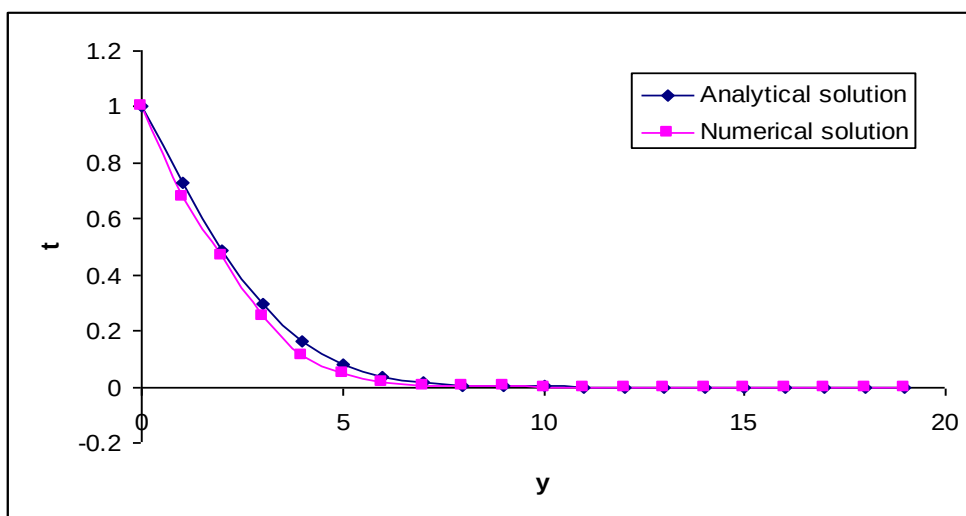
Fig.2. Comparison of Temperature Profiles when P_r=0.7333
